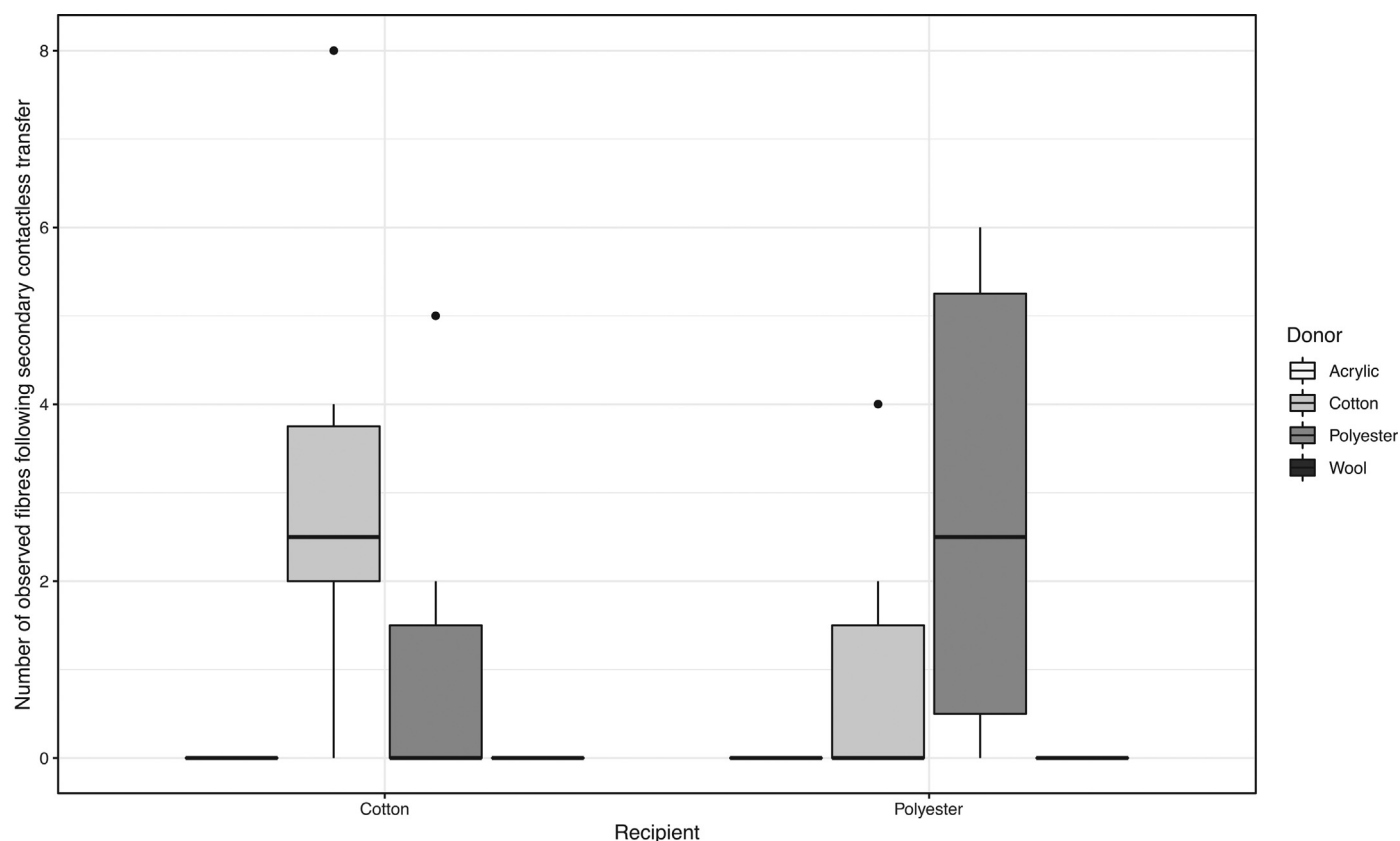
Fig. 5. Boxplots of the number of fibres counted after the secondary transfer experiments as a function of the composition of the donor and recipient garments.
